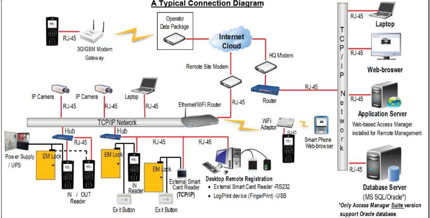
A Typical Connection Diagram
